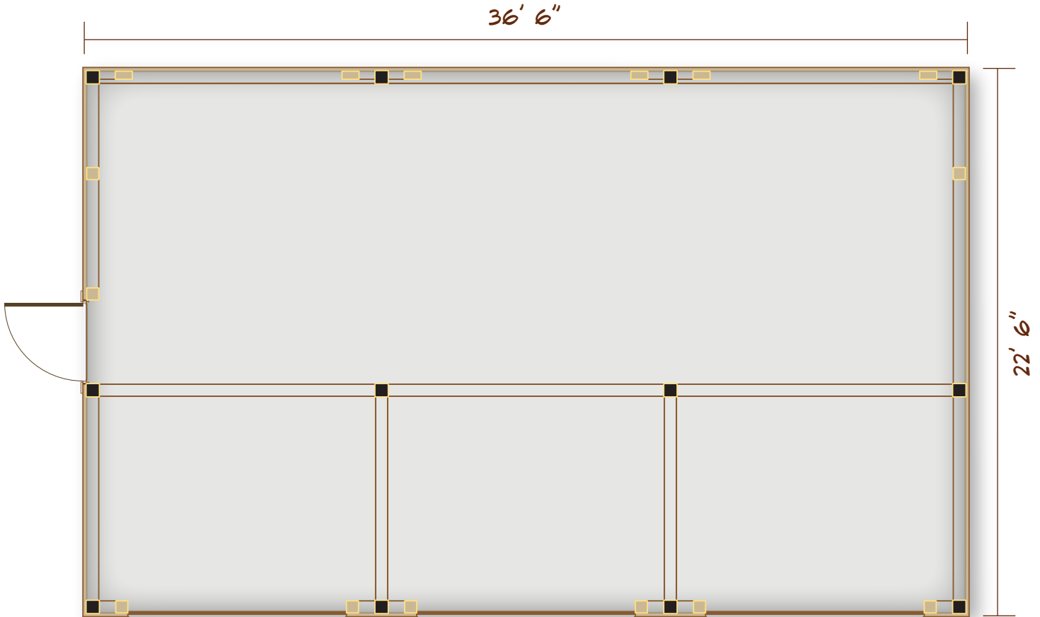
MAIN FLOOR PLAN 821 SF
